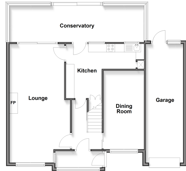
Ground Floor Approx. 67.9 sq. metres (730.6 sq. feet)
