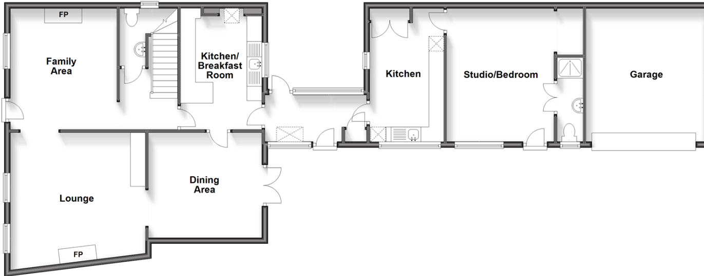
Ground Floor Approx. 126.0 sq. metres (1356.5 sq. feet)
