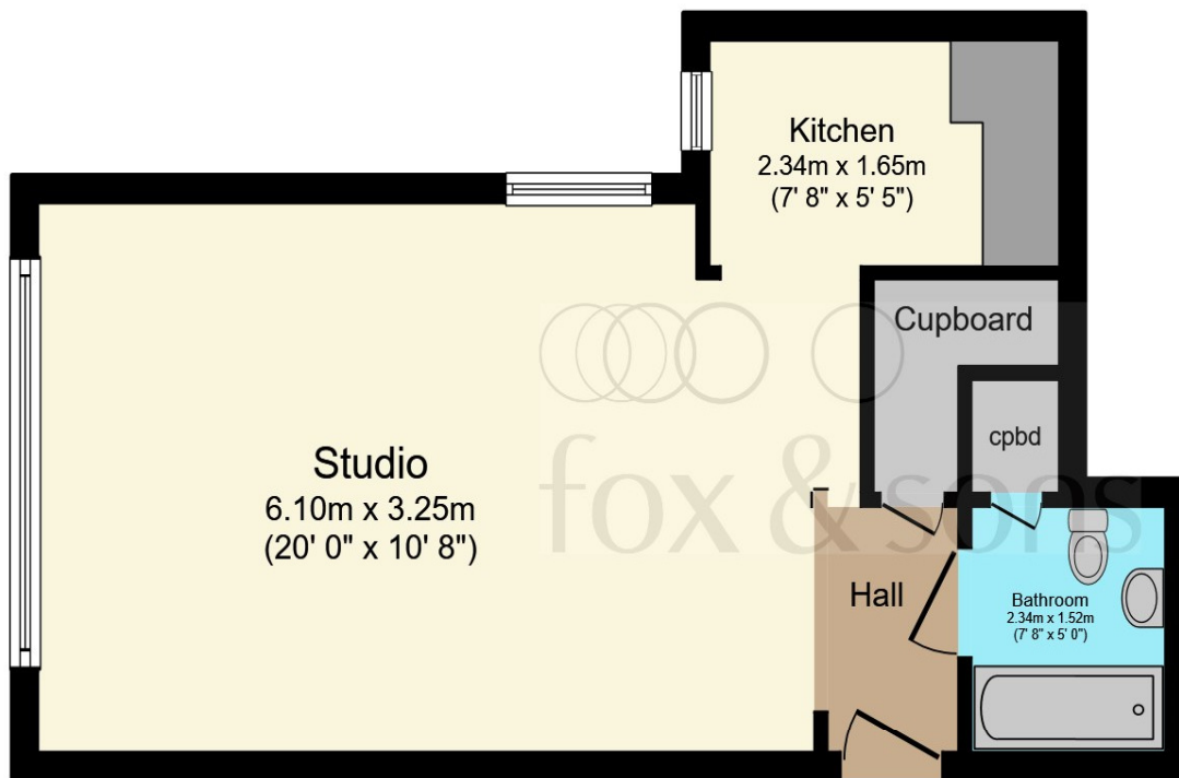
Floor Plan
