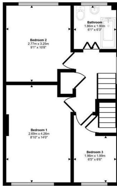
First Floor Approx 37 sq m / 398 sq ft
