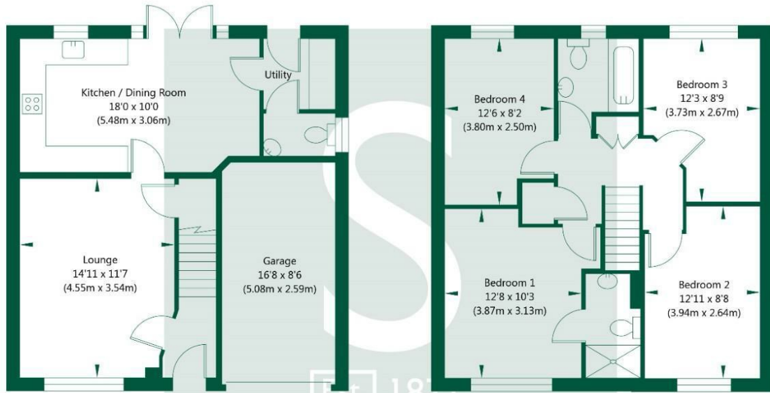
Ground Floor - (Excluding Garage) GROSS INTERNAL FLOOR AREA APPROX. 454 SQ FT / 42.15 SQ M
