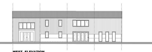
WEST ELEVATION.
