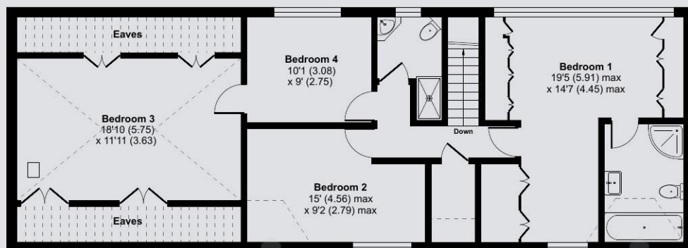
FIRST FLOOR
