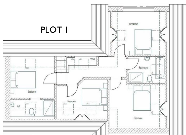
First Floor Plan Plot 1
