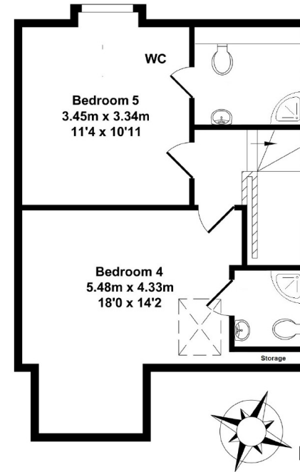
Second Floor Approx. Floor Area 38.72 Sq.M. (417 Sq.Ft.)
