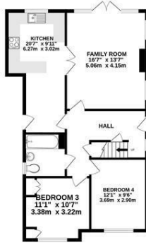
GROUND FLOOR 799 sq.ft. (73.3 sq.m.) approx.
