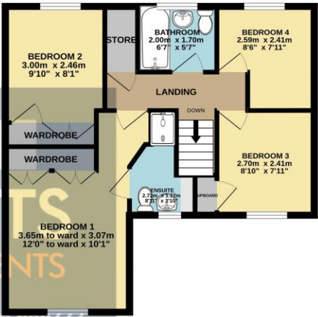
1ST FLOOR 48.8 sq.m. (526 sq.ft.) approx.
