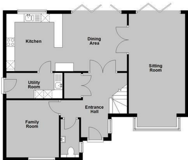
Ground Floor Approx. 77.7 sq. metres (836.5 sq. feet)
