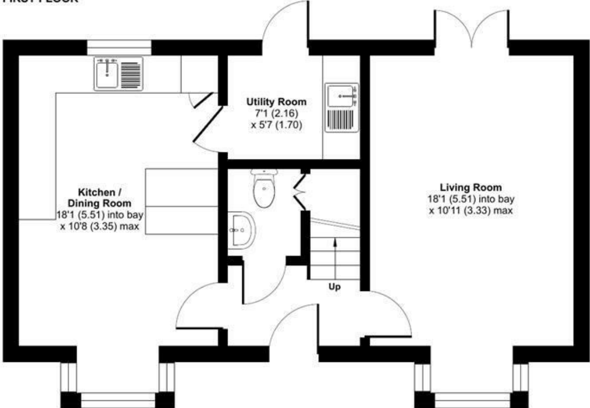
GROUND FLOOR
