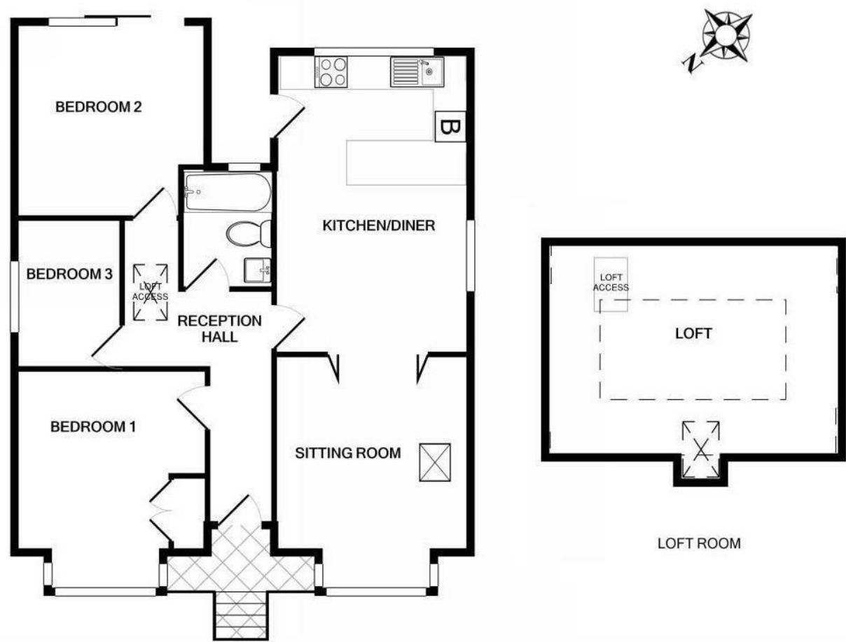
GROUND FLOOR
