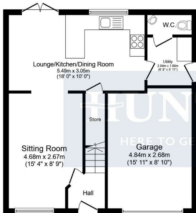
Ground Floor Floor area 57.5 sq.m. (619 sq.ft.)
