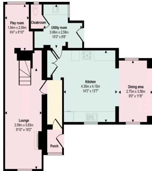
Ground Floor Approx 75 sq m / 805 sq ft
