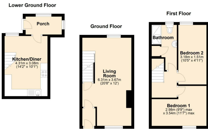
Floorplans are for identification purposes only and not to scale. Where measurements are shown, these are approximate and should not be relied on. Sanitary ware and kitchen fittings are representative only and approximate to actual shape, position and style. No liability is accepted in respect of any consequential loss arising from the use of this plan. Reproduced under licence from William Morris Energy Assessments. All rights reserved. Plan produced using PlanUp.
