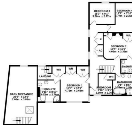
1ST FLOOR 1405 sq.ft. (130.5 sq.m.) approx.
