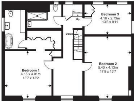
First Floor 1
