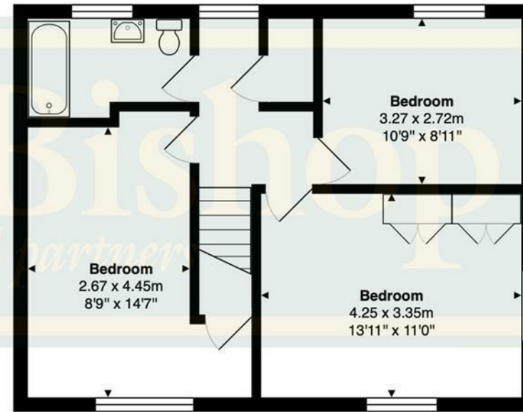
First Floor Area: 50.7 m 2 ... 546 ft 2
