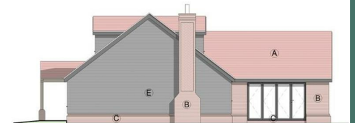
Proposed Side B Elevation 1:100
