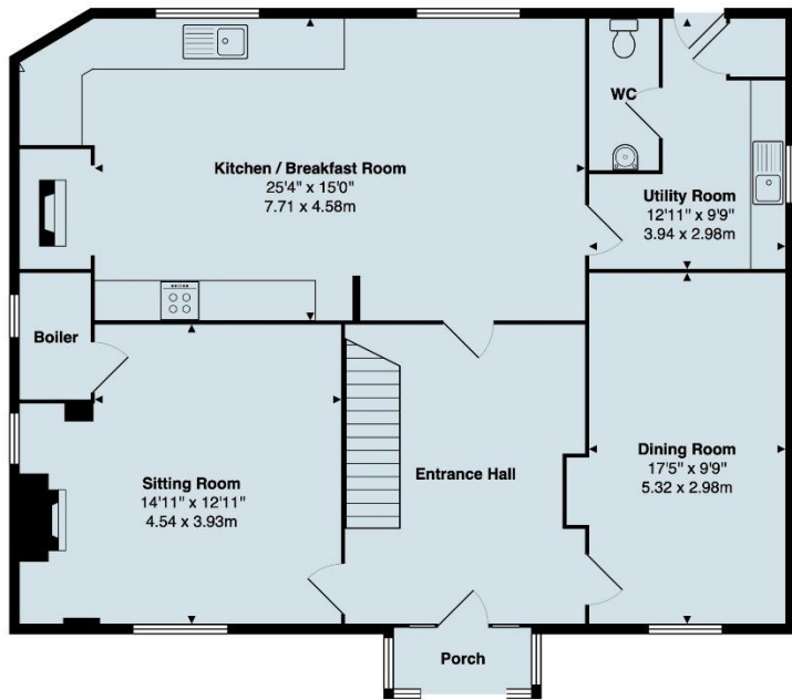
Ground Floor Area: 1144 ft 2 ... 106.3 m 2
