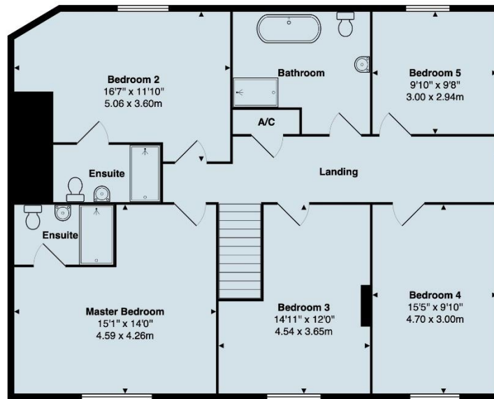
1st Floor Area: 1144 ft 2 ... 106.3 m 2
