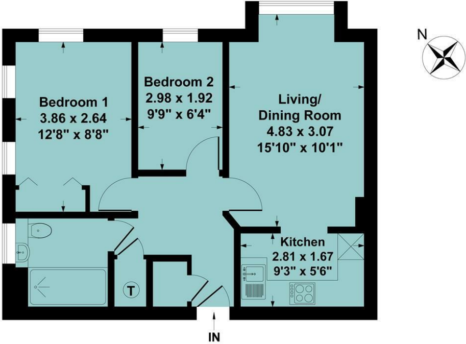
Second Floor
