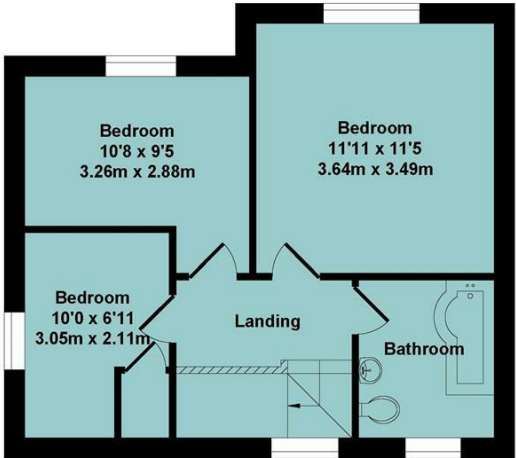
Total Approx. Floor Area 1147 Sq.Ft. (106.50 Sq.M.) All items illustrated on this plan are included in the "Total Approx Floor Area"
