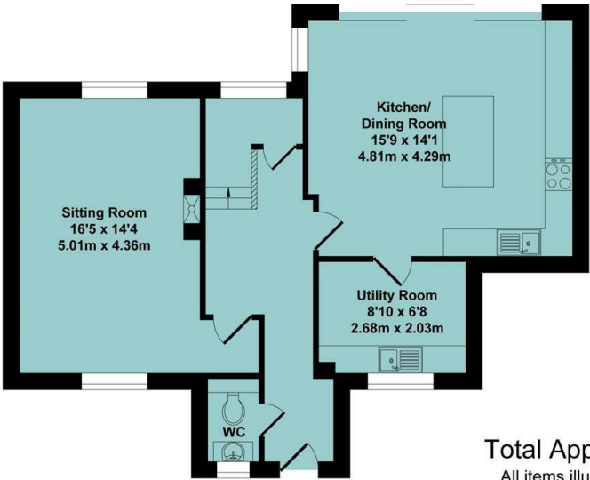
Ground Floor Approx. Floor Area 611 Sq.Ft. (56.80 Sq.M.)
