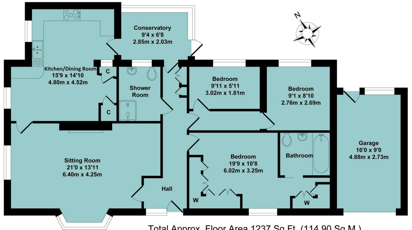
Total Approx. Floor Area 1237 Sq.Ft. (114.90 Sq.M.) All items illustrated on this plan are included in the "Total Approx Floor Area"
