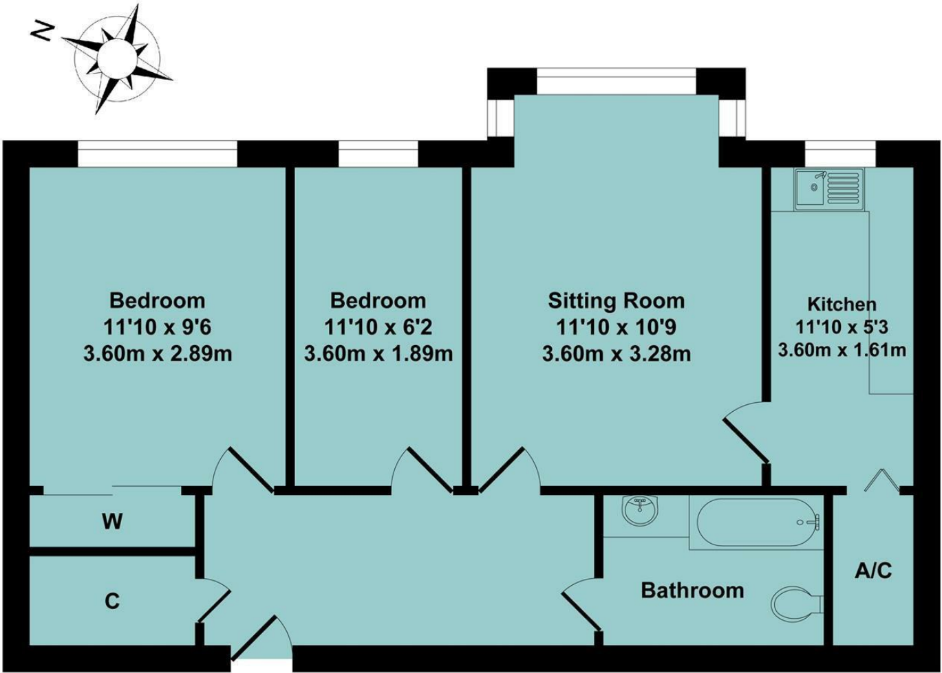
Total Approx. Floor Area 600 Sq.Ft. (55.70 Sq.M.) All items illustrated on this plan are included in the "Total Approx Floor Area"
