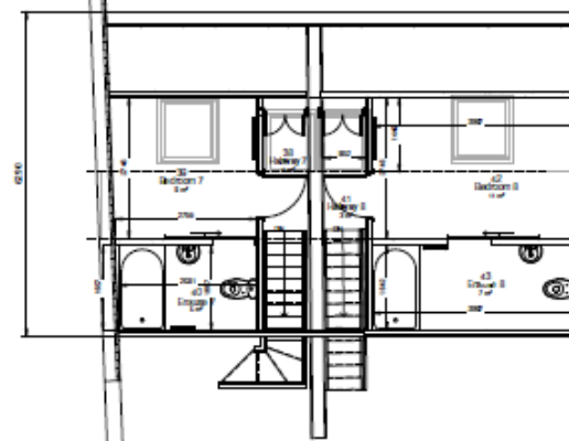
4 SF - Partition Layout 1:50
