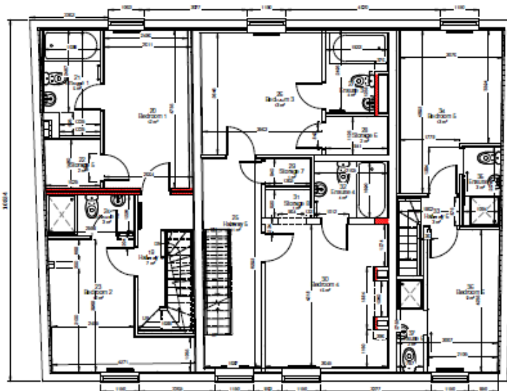
3 FF - Partition Layout 1:50
