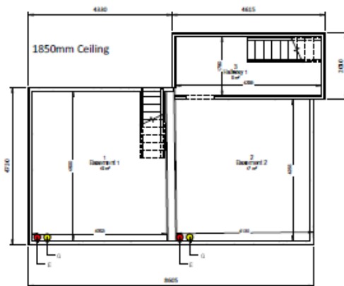
1 Basement - Partition Layout 1:50
