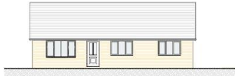
East Elevation Scale 1:50
