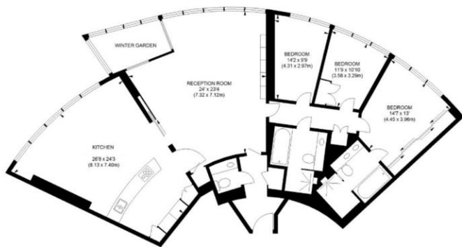
APPROX. GROSS INTERNAL FLOOR AREA 1639 SQ FT / 152.76 SQ M
