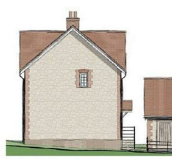
Dwelling 3 - South Elevation 1:50
