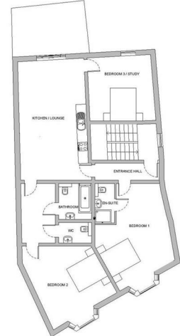
FIRST FLOOR PLAN FLAT 1
