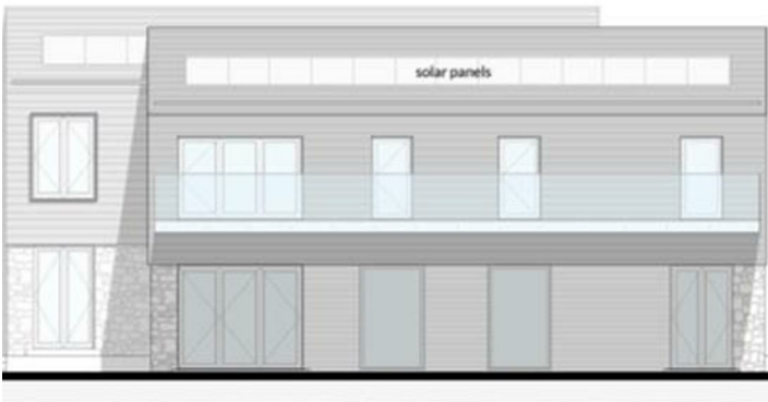
South Elevation 1:100
