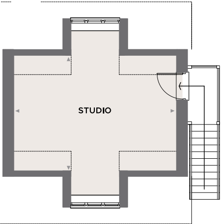
NO.4 STUDIO OVER DOUBLE GARAGE Refer to site plan for location
