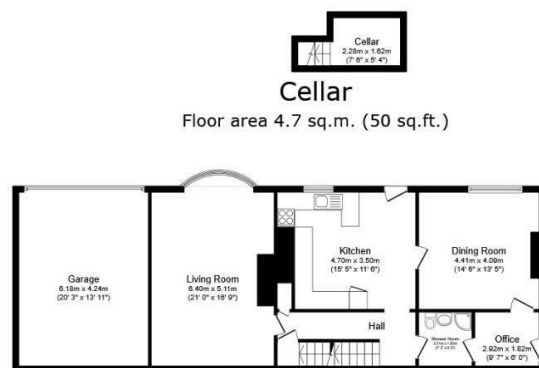
Ground Floor Floor area 104.8 sq.m. (1,128 sq.ft.)
