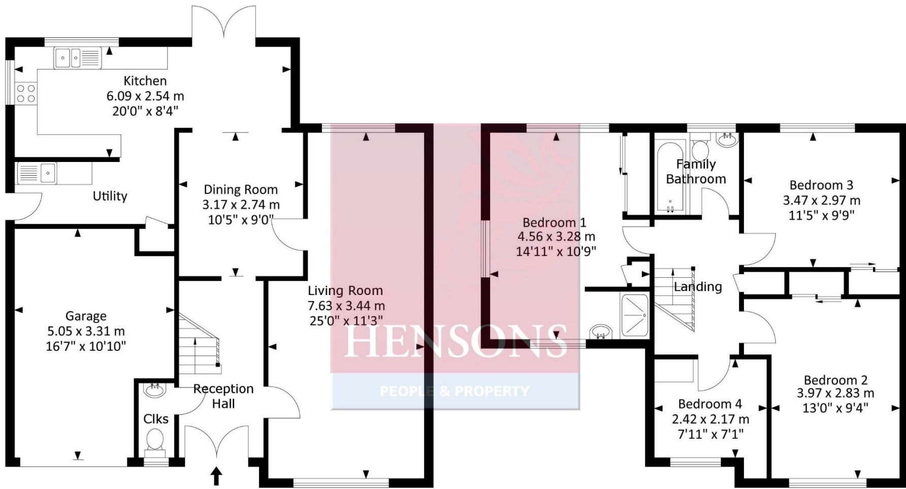
Ground Floor
