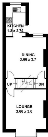
GROUND FLOOR
