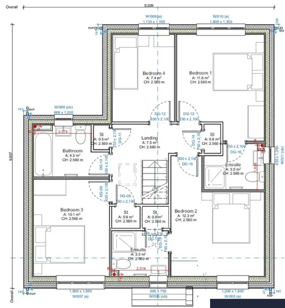
Total floor area 134 sqm / 1442 sqft
