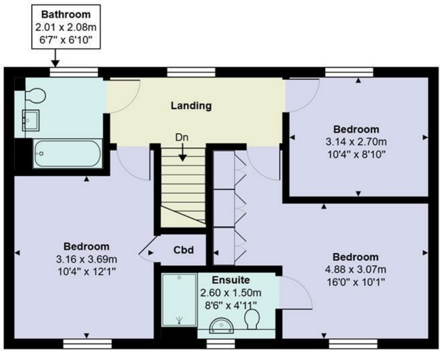
First Floor Area: 55.6 m 2 ... 598 ft 2
