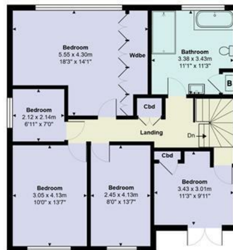
First Floor Area: 84.7 m 2 ... 912 ft 2
