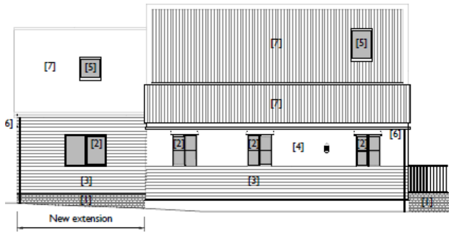
SOUTH-EAST ELEVATION
