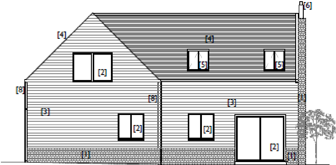
NORTH-WEST ELEVATION
