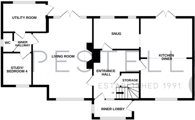
GROUND FLOOR 983 sq.ft. (91.3 sq.m.) approx.
