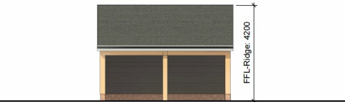
Front Elevation
