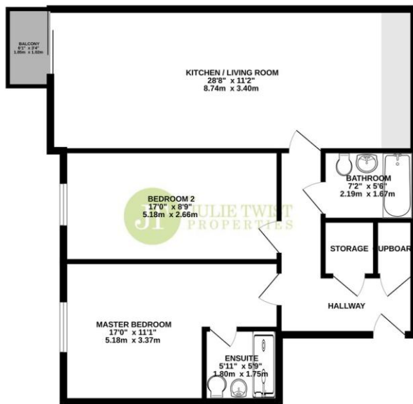
FOURTH FLOOR 811 sq.ft. (75.3 sq.m.) approx.
