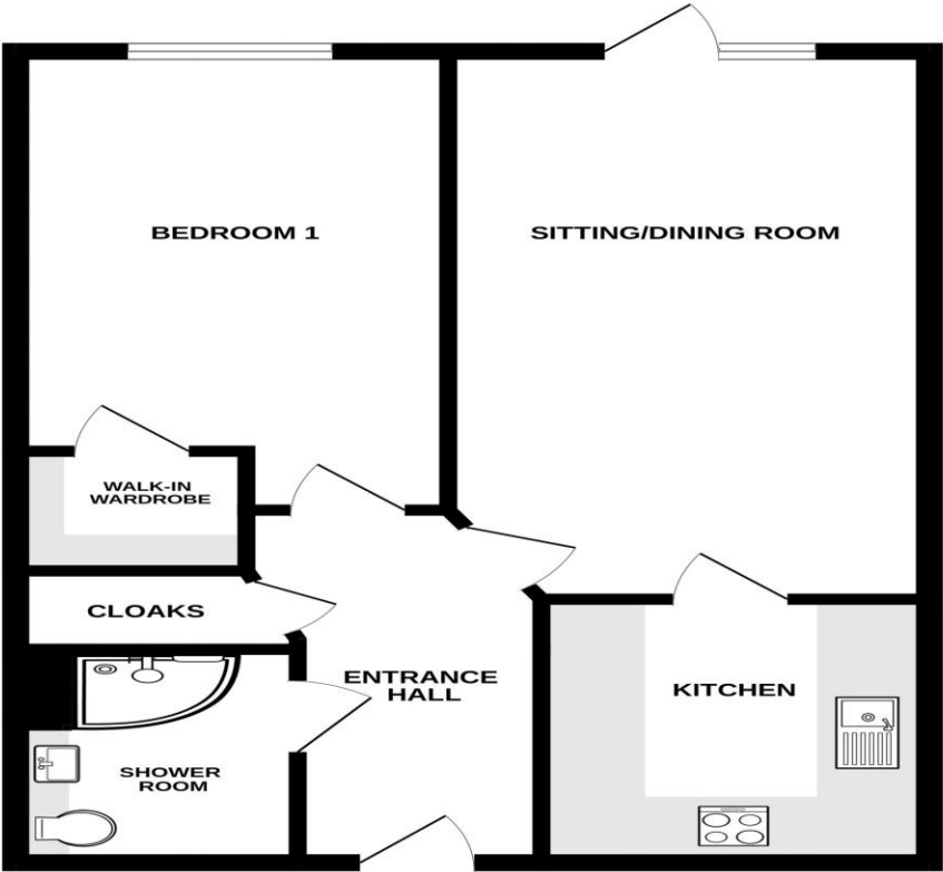
GROUND FLOOR 564 sq.ft. (52.4 sq.m.) approx.
