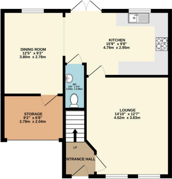
GROUND FLOOR 560 sq.ft. (52.1 sq.m.) approx.
