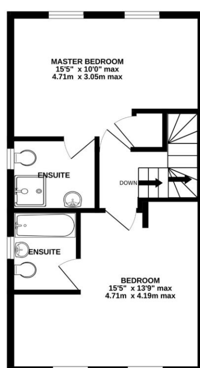
2ND FLOOR 441 sq.ft. (41.0 sq.m.) approx.
