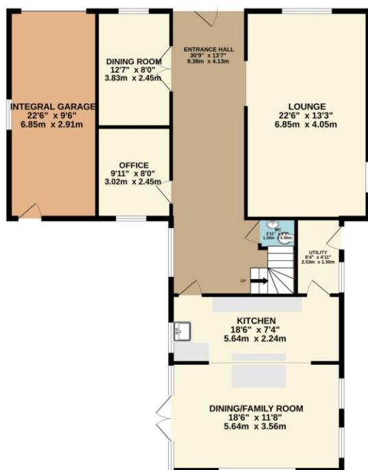
GROUND FLOOR 1381 sq.ft. (128.3 sq.m.) approx.
