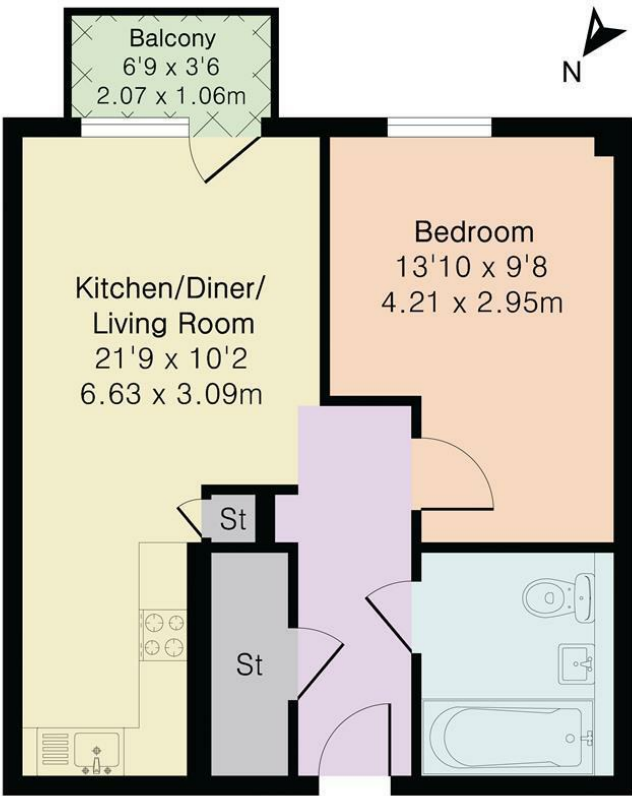
First Floor Apartment
