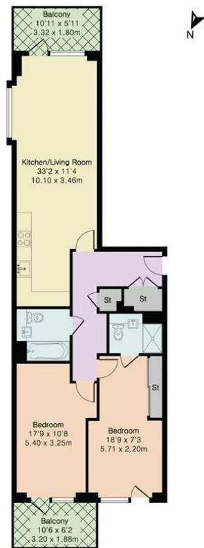
Fifth Floor
